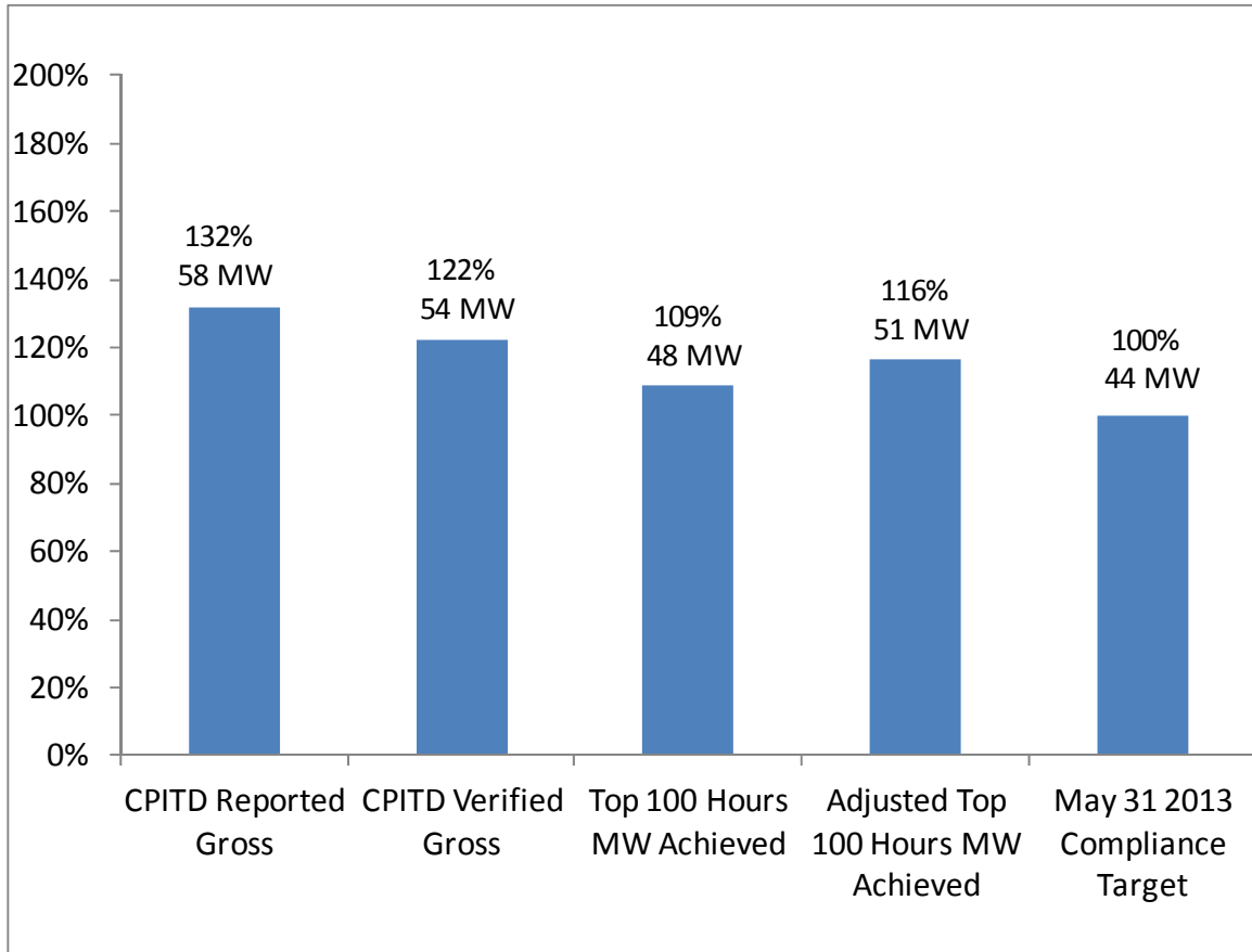
Figure 1-2. Portfolio CPITD Peak Demand Reduction
